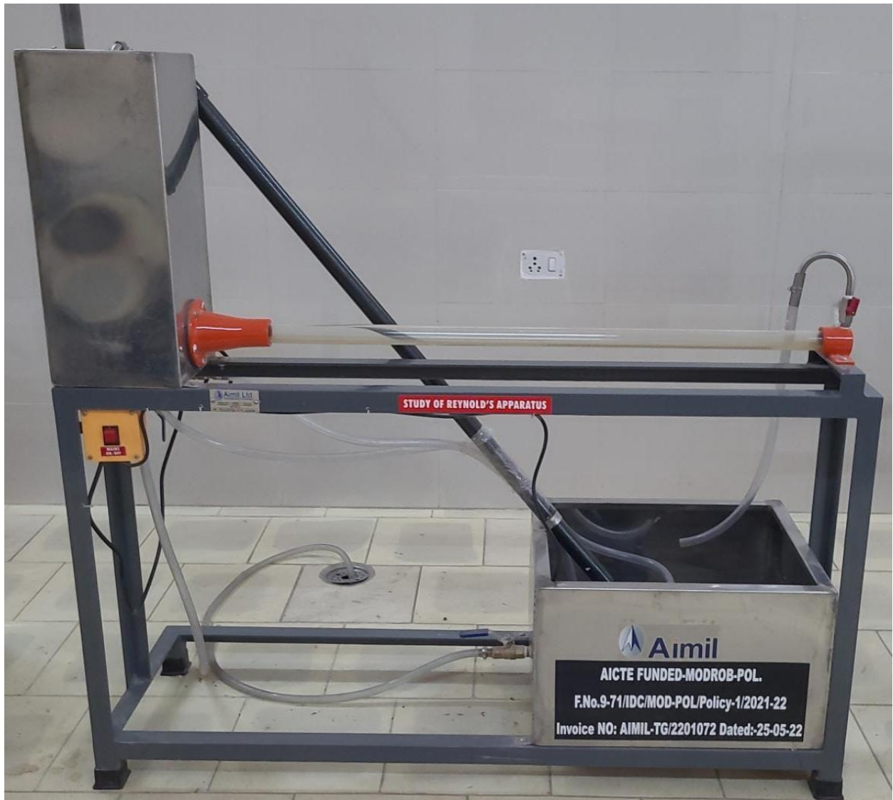
Reynold's Apparatus
